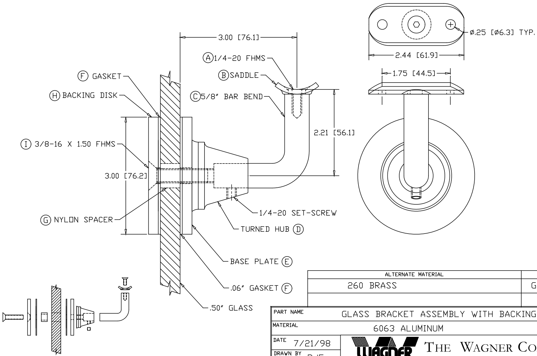
EXPLODED VIEW
