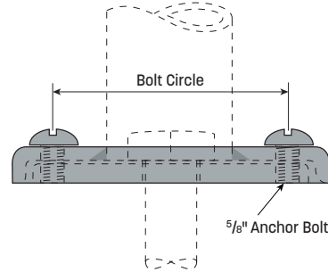
Floor Flange with Anchor Plate.
