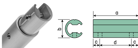
3393 Drill Holes as Shown for 1/4" Set Screw .
